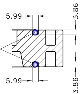
Section view B-B
