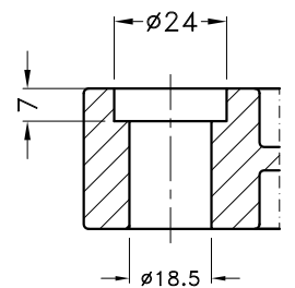
Section view A-A
